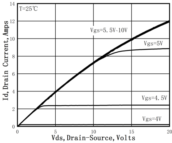
Figure 1. On-Region Characteristics
