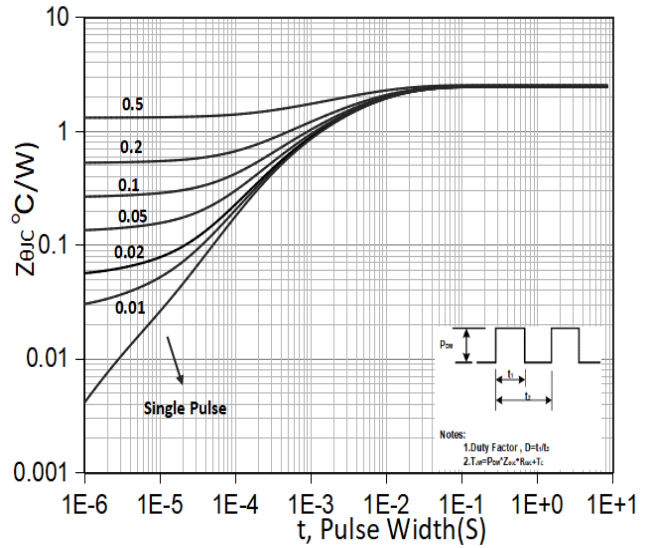
Figure 10. Transient Thermal Response Curve (TO-220F)
